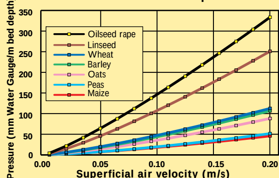
Figure 2. Pressure resistance curves for seven crops
