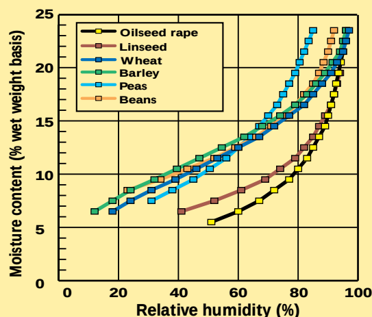
Figure 1. Relative humidity / moisture content relationships for six crops at 15°C
